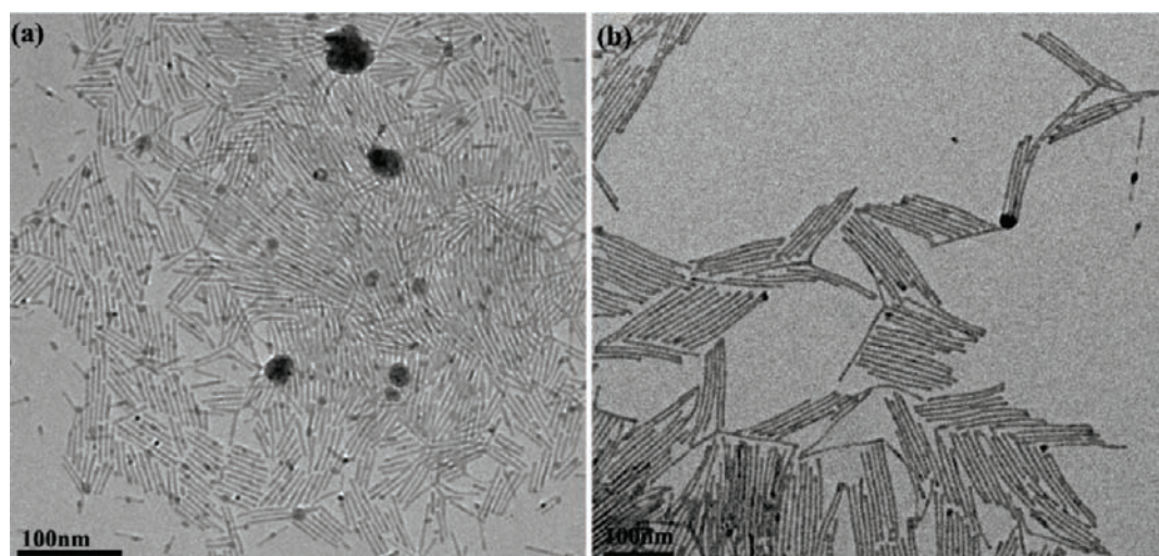
Figure 7. (a) Silver Sulfide (Ag 2 S) nanorods prepared by cation exchange from CdS. (b) Elongated Ag 2 S after a two amine washes with an average length of ~120 nm.
