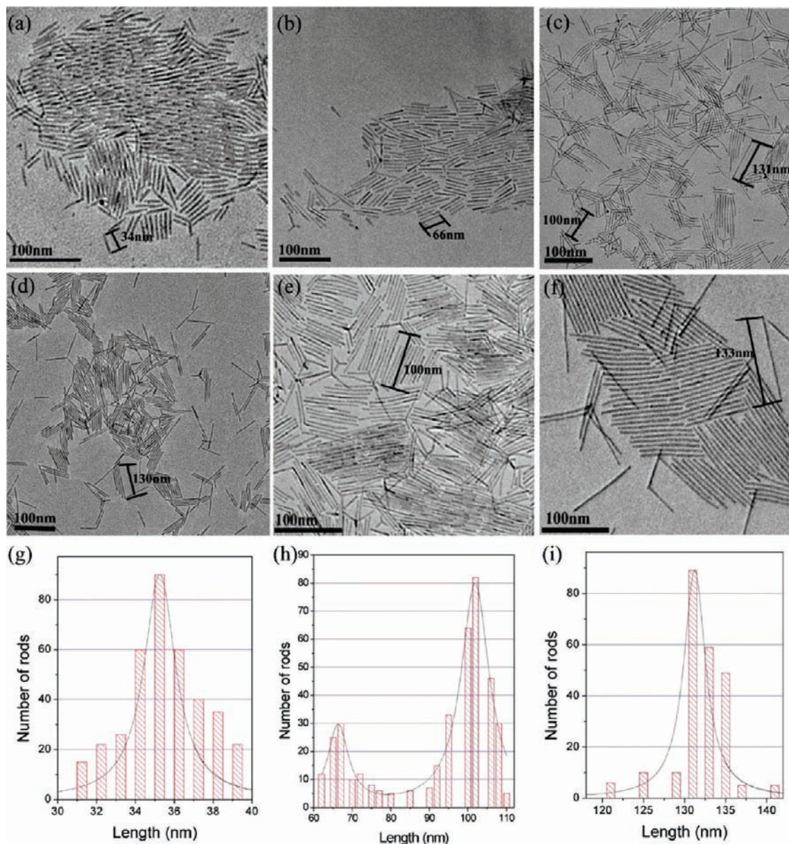
Figure 1. (a) TEM images of as synthesized CdS nanorods. (b) Elongated nanorods after a 30 s immersion in octylamine. (c) Elongated nanorods after a 120 s immersion in octylamine. (d) Elongated nanorods after a 30 s immersion in high concentration (0.030 mol) of octylamine. (e) Elongation after 30 s agitation in the presence of octylamine. (f) Elongation was observed after further addition of amine (0.018 mol) leading to monodispersed nanowires. Size distribution curves (g) correspond to the as synthesized nanorods showing the mean length of 34 nm, (h) corresponds to image e showing that the elongation is bimodal with some of the nanorods doubling and some tripling in length. (i) Size distribution curve of monodispersed nanorods imaged corresponding to image f .
