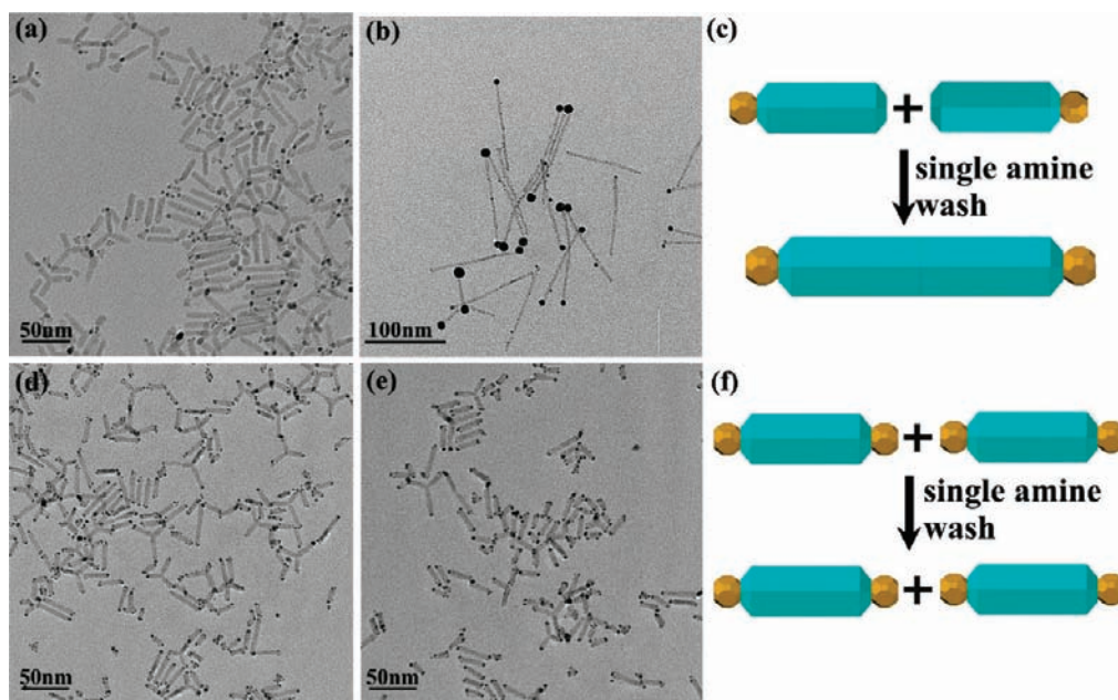
Figure 5. (a) CdS nanorods where gold is asymmetrically grown onto the (001) facets. (b) When subjected to octylamine it resulted in the attachment of these nanorods at the untipped side. (c) Schematic showing the attachment of the gold tipped nanorods due to a single octylamine wash. (d) CdS nanorods with symmetric gold growth onto the (001) facets. (e) When amine was added no attachment was seen. (f) Schematic showing the result of an amine wash on symmetric gold tipped nanorods resulting in no elongation due to the capping of the facets.
