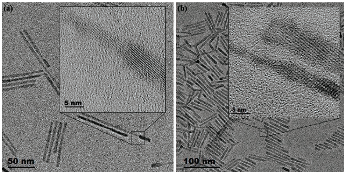
Figure 4. (a) TEM image of two different diameters nanorods attaching, with HRTEM insets magnifying the joining area. (b) TEM analysis of two nanorods with different diameters attaching leading to the occurrence of stacking fault.
