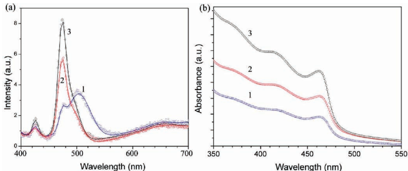
Figure 6. (a) Photoluminescence and (b) UV-vis measurements of the as-prepared CdS nanorods (curve 1), elongated nanorods after washing with low concentration (0.006 mol) octylamine (curve 2), and high concentration (0.024 mol) octylamine (curve 3).
