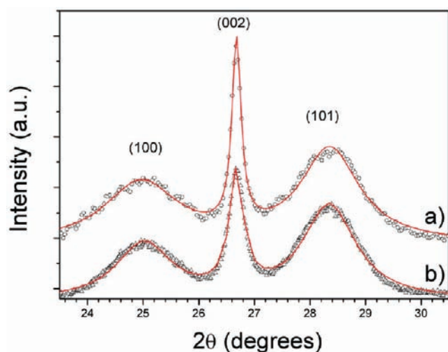
Figure 3. XRD spectra (a) nanorods subsequent to low concentration amine (0.018 mol) wash (b) as synthesized nanorods.
