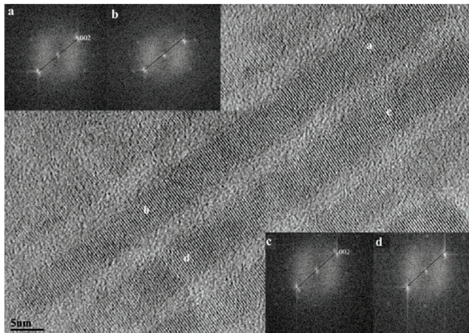
Figure 2. High resolution TEM montage image of elongated nanorods, with selected area FFT insets. The letters in the FFT inset correspond to the area on the nanorod where the FFT measurement was taken from respectively and lines have been inserted and mirrored onto the adjoining image to further show the change in crystal direction.
